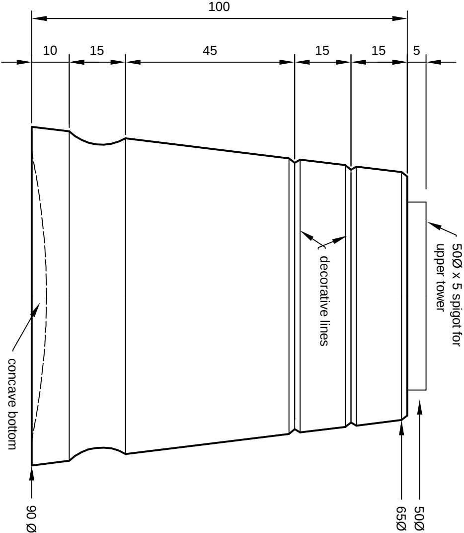
LOWER TOWER Scale: full size
