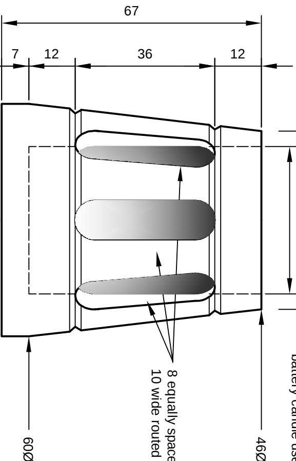
LAMP ROOM Scale: full size
