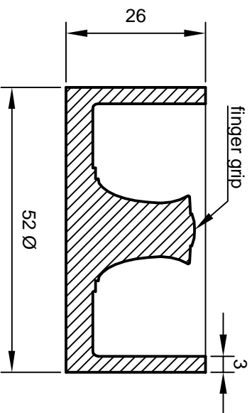
TRAY (section)
