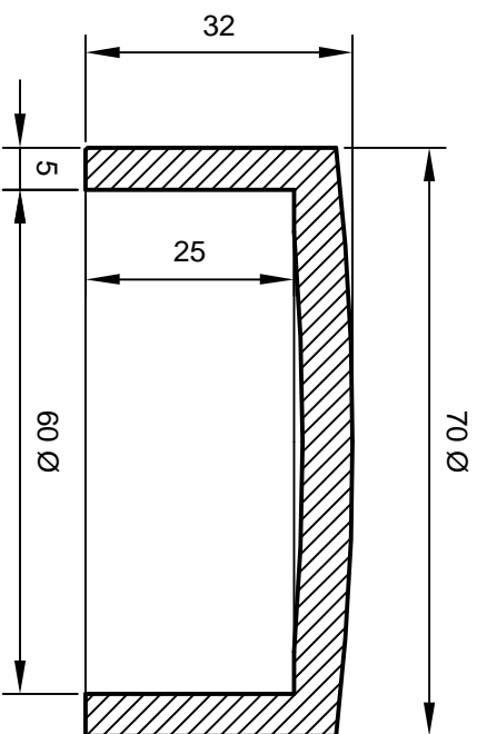
LID (section)
