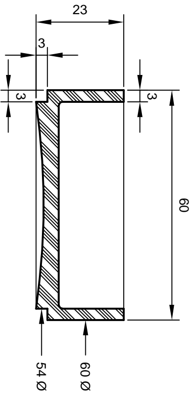
The Boxes scale: full size (3 required)
